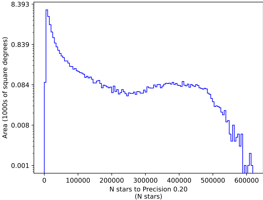
too_ignore_5_1v3.4_10yrs z: N stars to Precision 0.20
