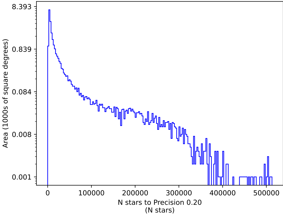
too_ignore_5_1v3.4_10yrs u: N stars to Precision 0.20
