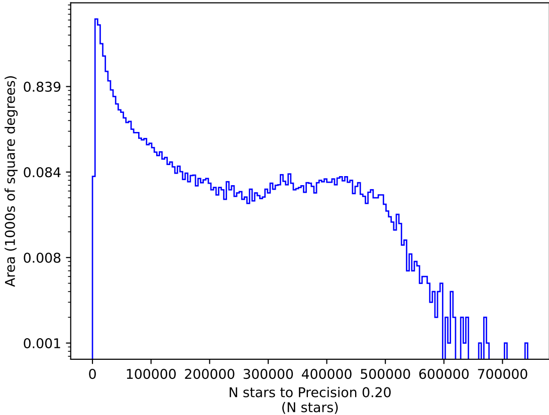
too_ignore_5_1v3.4_10yrs r: N stars to Precision 0.20
