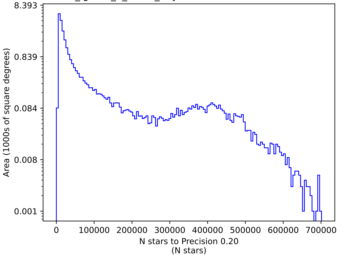
too_ignore_5_1v3.4_10yrs i: N stars to Precision 0.20
