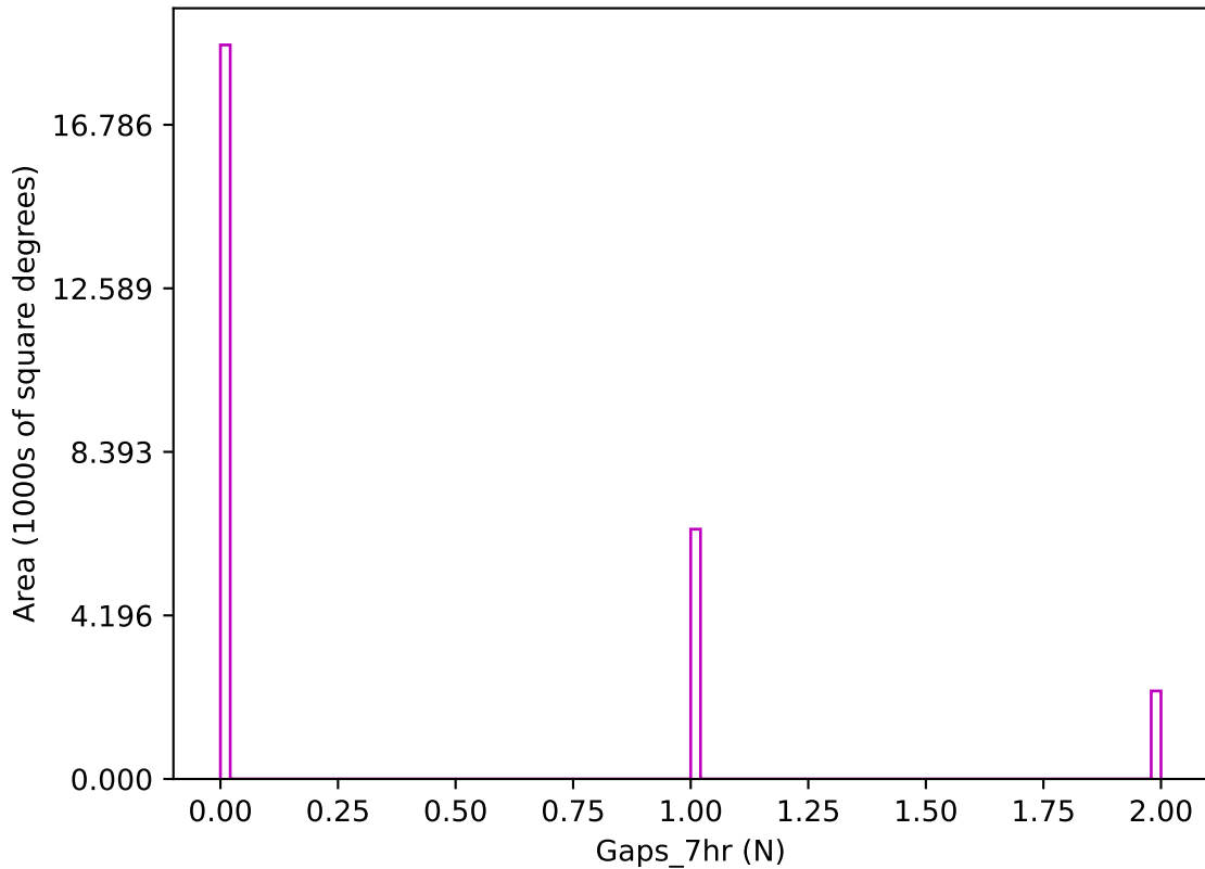
too_ignore_5_1v3.4_10yrs z band: Gaps_7hr
