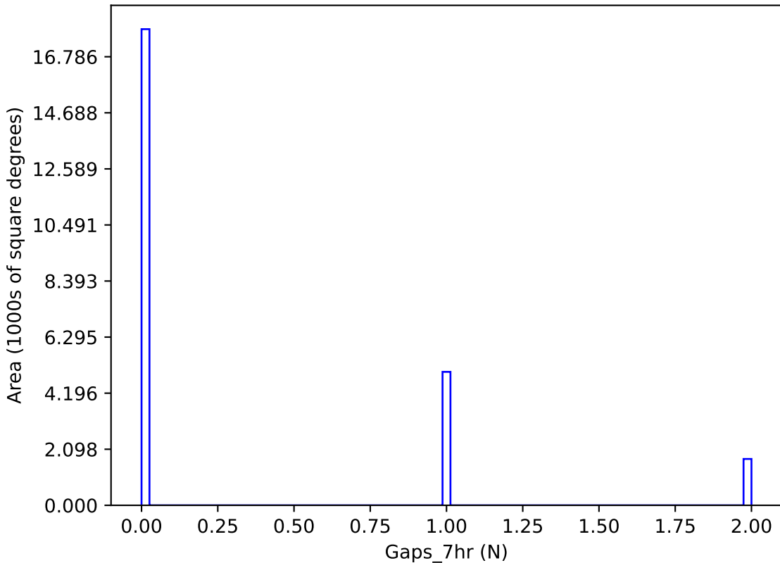
too_ignore_5_1v3.4_10yrs y band: Gaps_7hr
