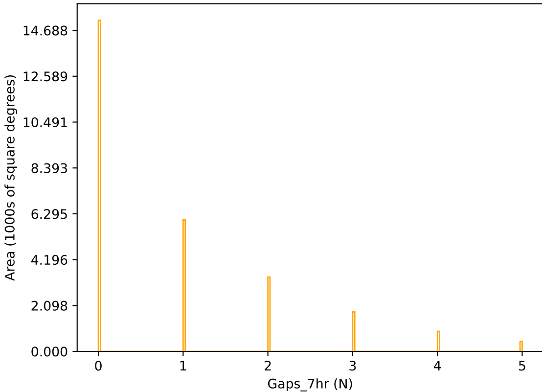
too_ignore_5_1v3.4_10yrs r band: Gaps_7hr
