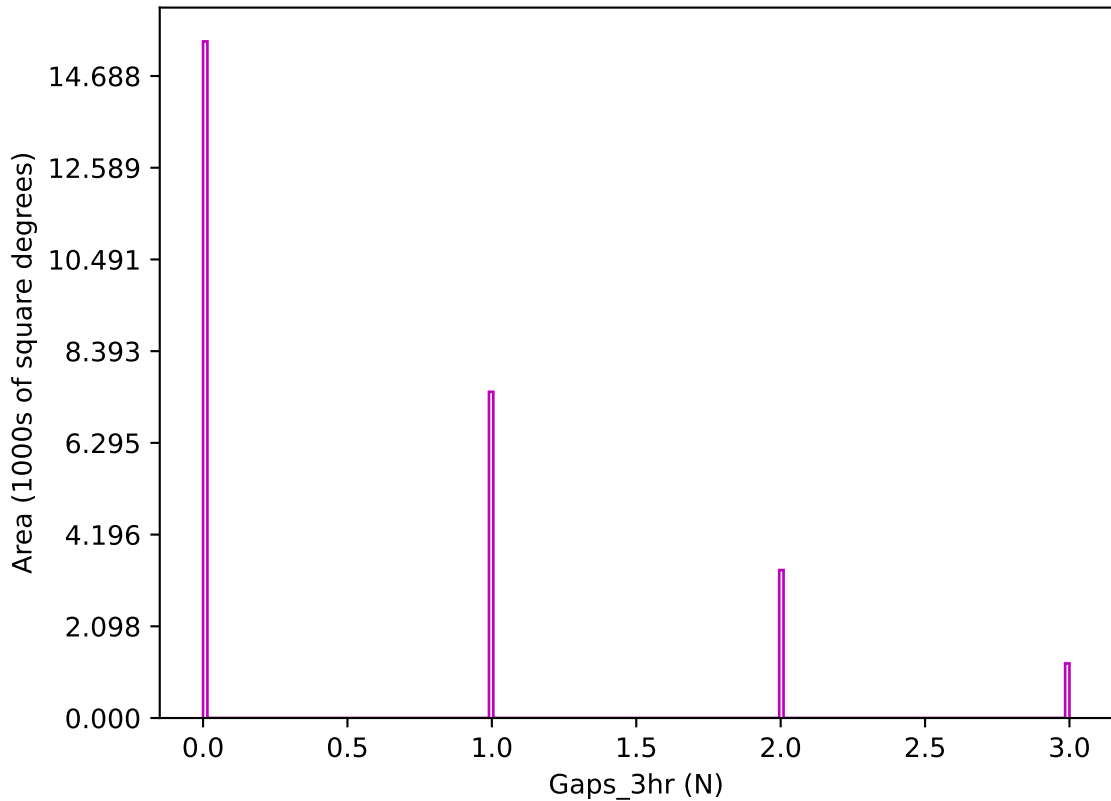
too_ignore_5_1v3.4_10yrs z band: Gaps_3hr
