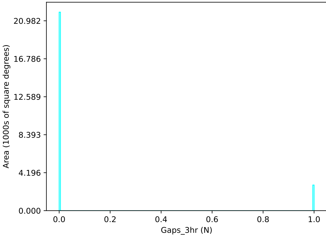
too_ignore_5_1v3.4_10yrs u band: Gaps_3hr
