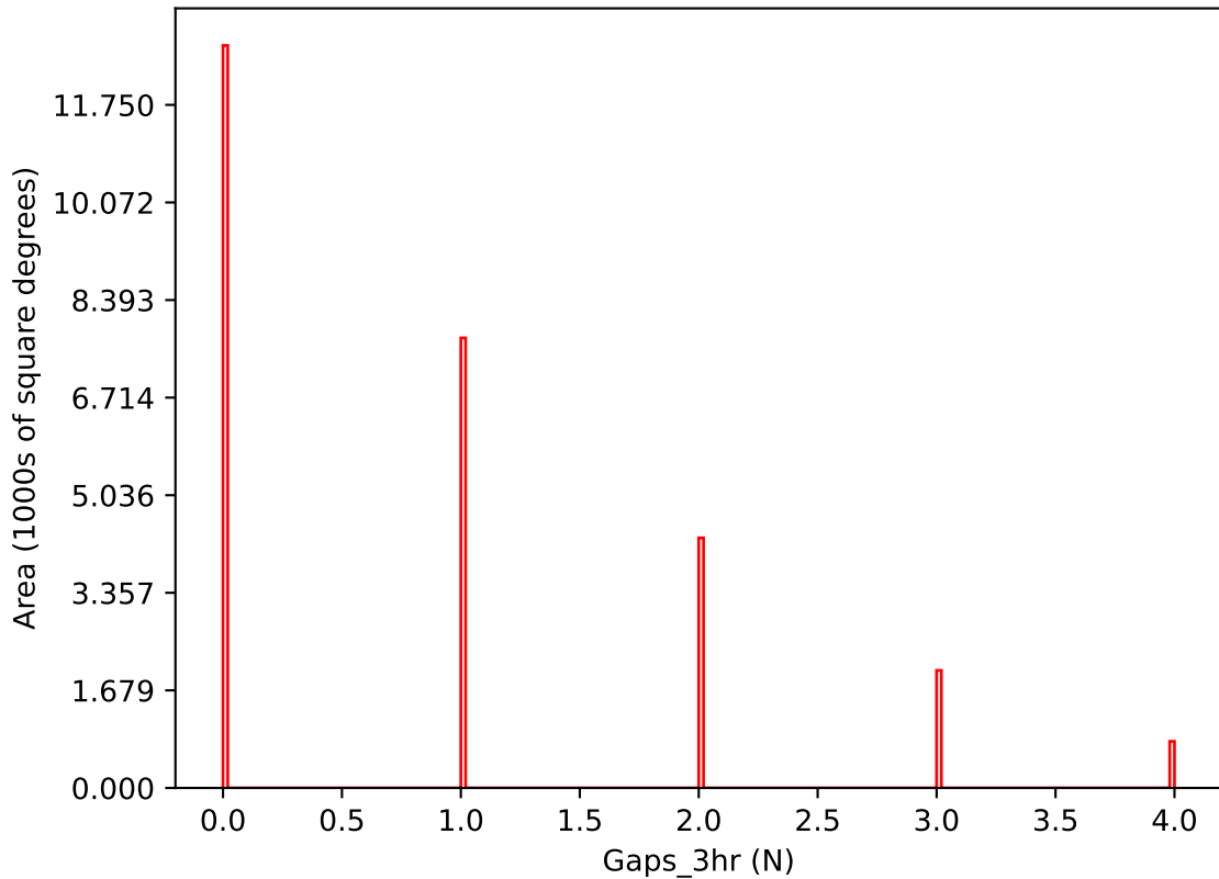
too_ignore_5_1v3.4_10yrs i band: Gaps_3hr
