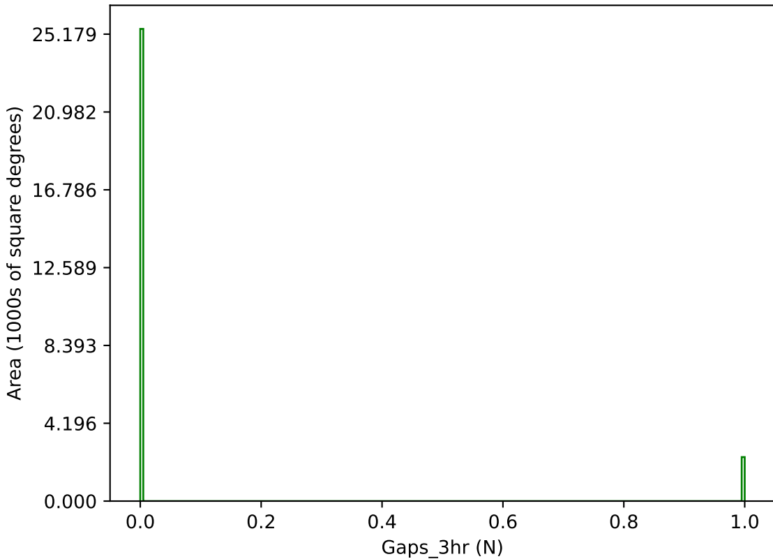
too_ignore_5_1v3.4_10yrs g band: Gaps_3hr
