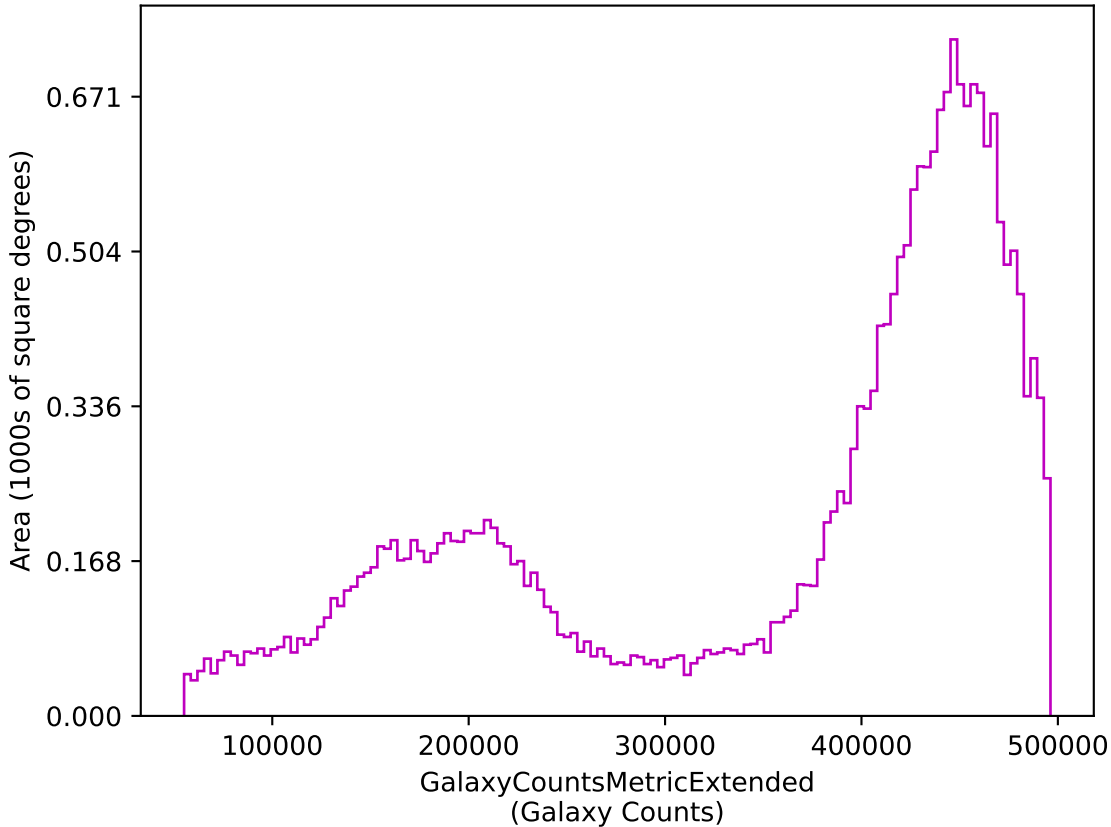
too_ignore_5_1v3.4_10yrs z: GalaxyCountsMetricExtended
