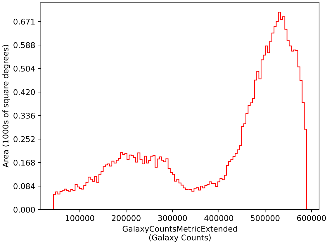
too_ignore_5_1v3.4_10yrs i: GalaxyCountsMetricExtended
