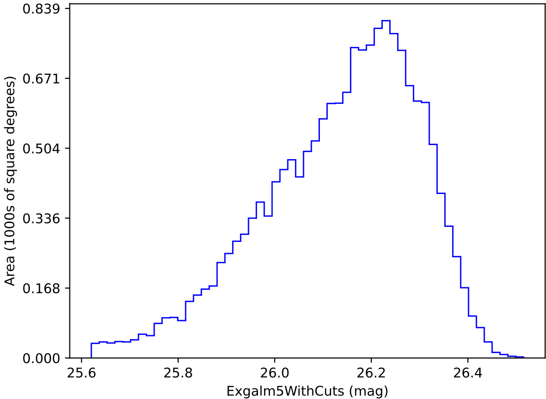
too_ignore_5_1v3.4_10yrs i band non-DD year 6: Exgal5WithCuts
