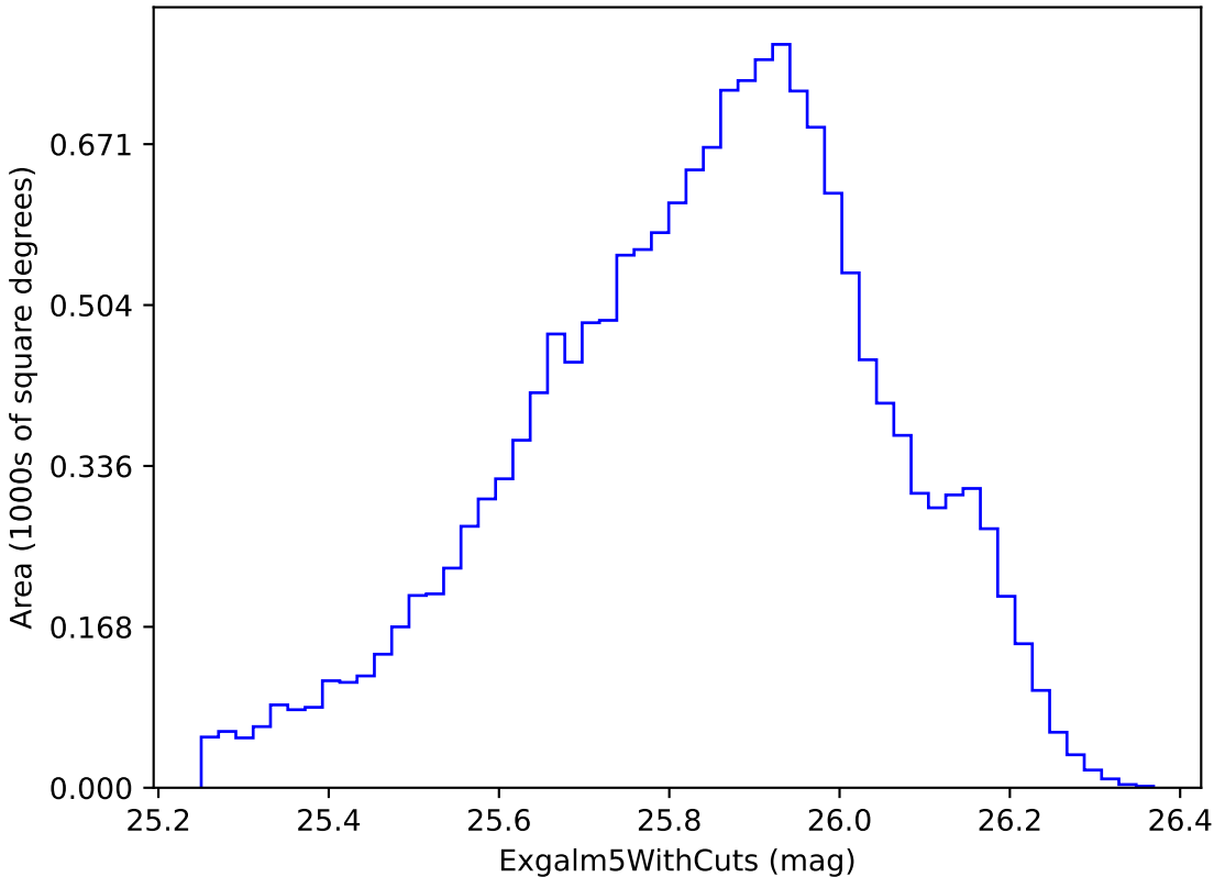
too_ignore_5_1v3.4_10yrs i band non-DD year 3: Exgal5WithCuts
