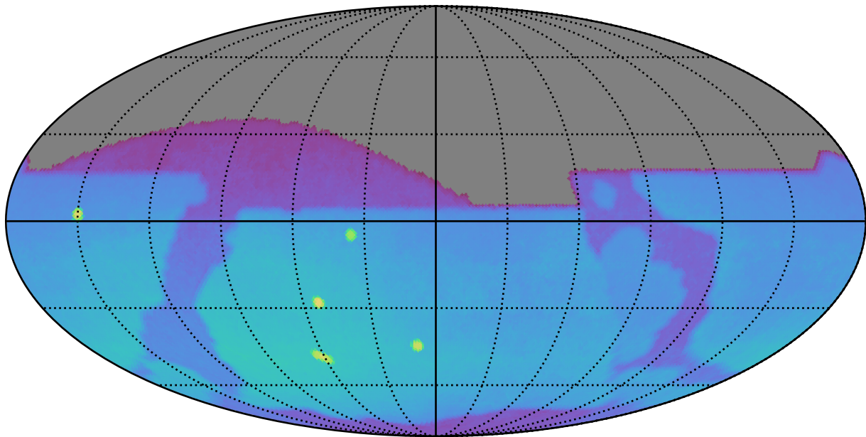
too_ignore_5_1v3.4_10yrs : Brown Dwarf, L7
