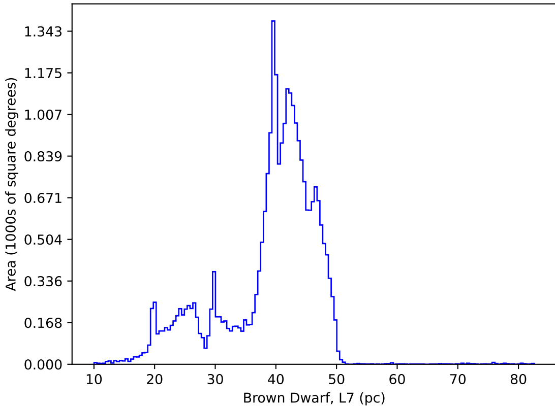
too_ignore_5_1v3.4_10yrs : Brown Dwarf, L7
