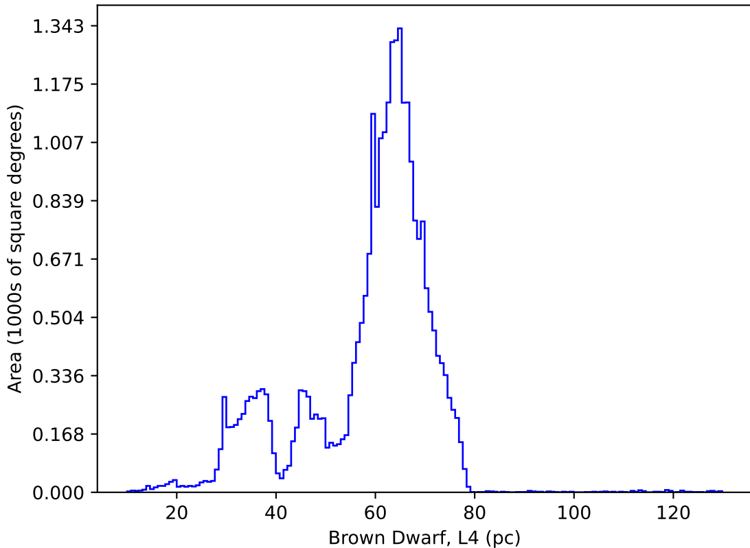
too_ignore_5_1v3.4_10yrs : Brown Dwarf, L4
