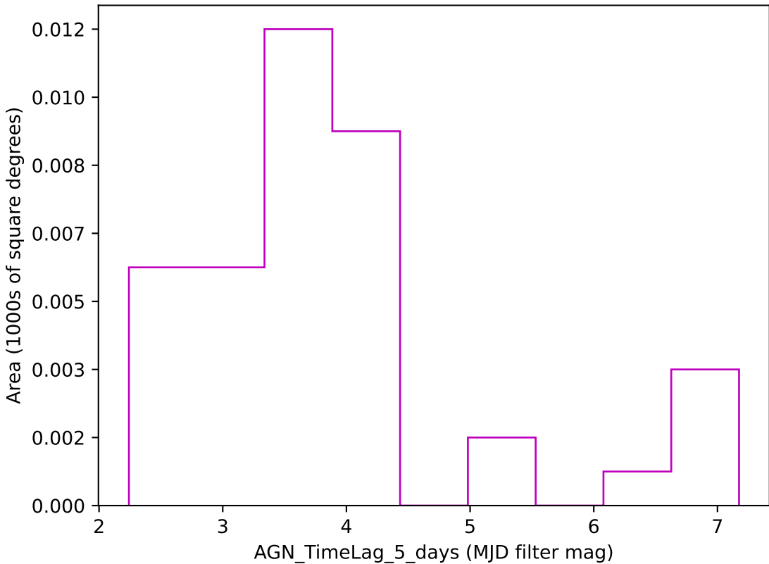
too_ignore_5_1v3.4_10yrs z band: AGN_TimeLag_5_days
