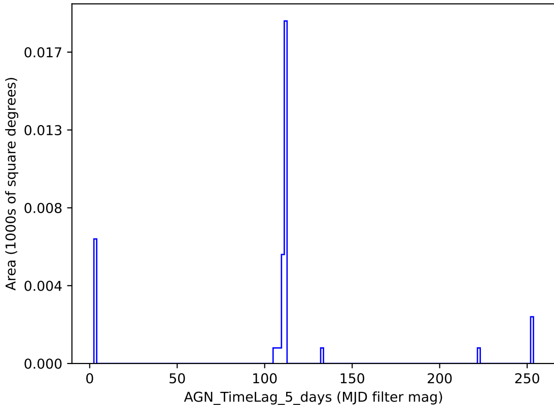
too_ignore_5_1v3.4_10yrs y band: AGN_TimeLag_5_days
