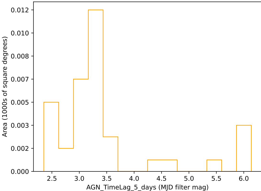
too_ignore_5_1v3.4_10yrs r band: AGN_TimeLag_5_days
