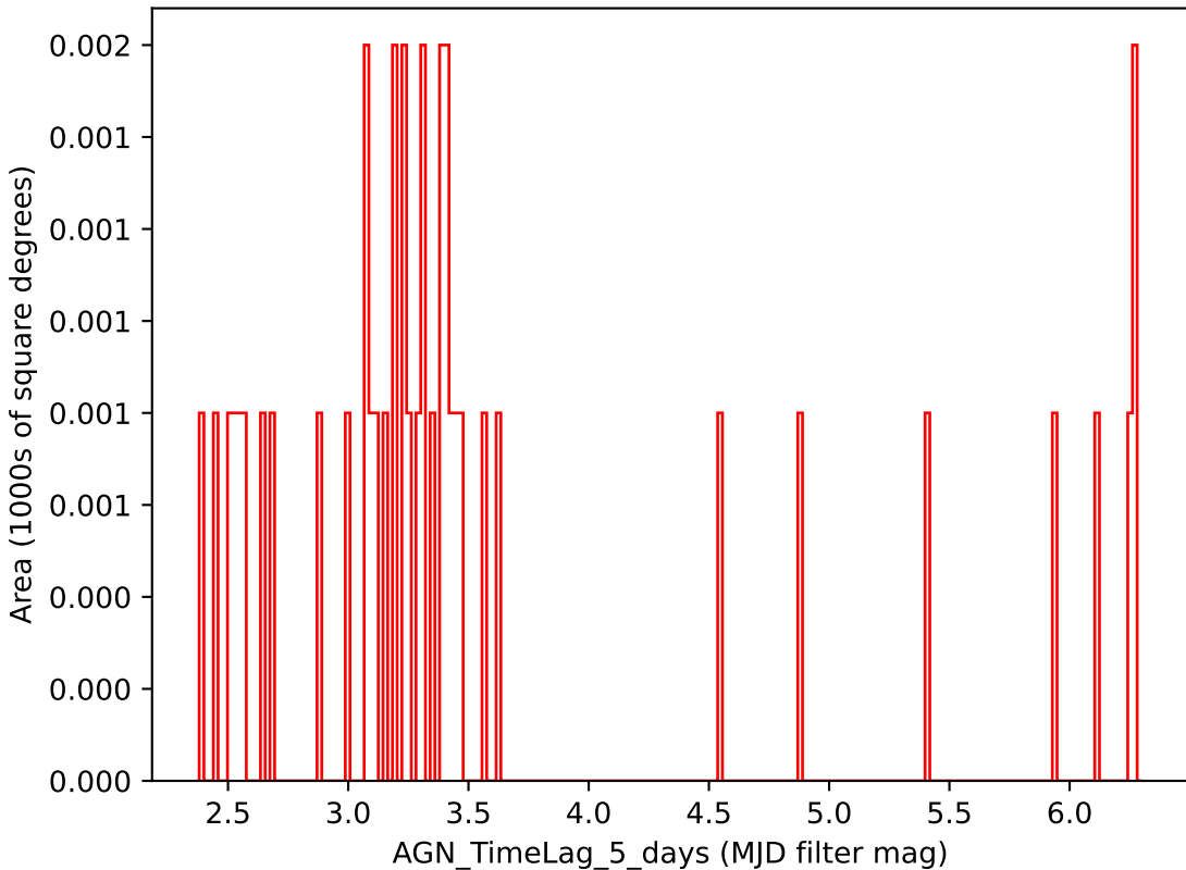
too_ignore_5_1v3.4_10yrs i band: AGN_TimeLag_5_days
