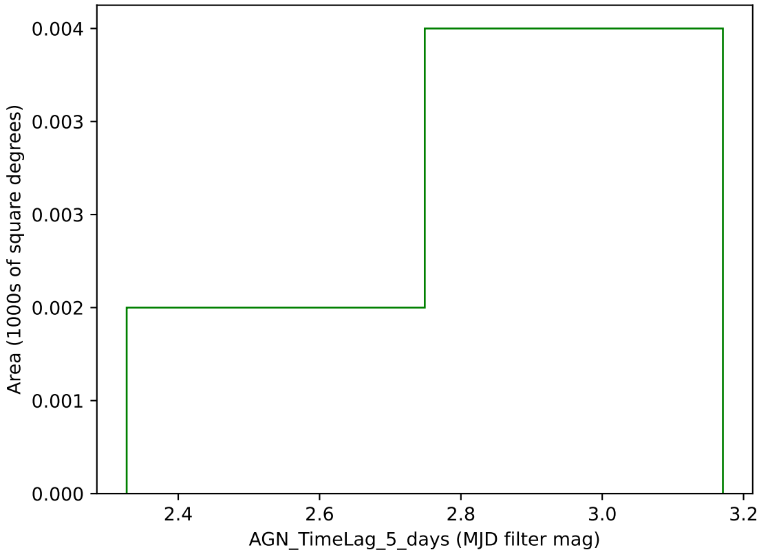
too_ignore_5_1v3.4_10yrs g band: AGN_TimeLag_5_days
