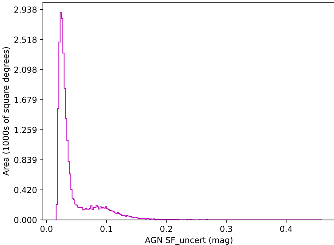
too_ignore_5_1v3.4_10yrs z band: AGN SF_uncert
