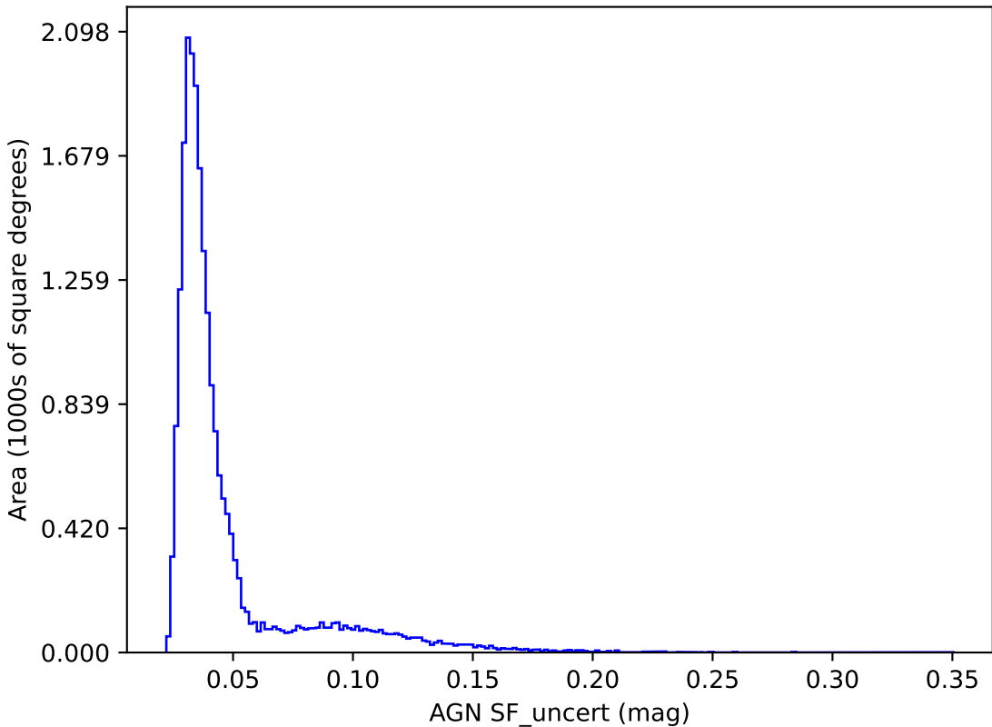
too_ignore_5_1v3.4_10yrs y band: AGN SF_uncert
