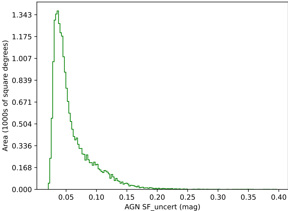
too_ignore_5_1v3.4_10yrs g band: AGN SF_uncert
