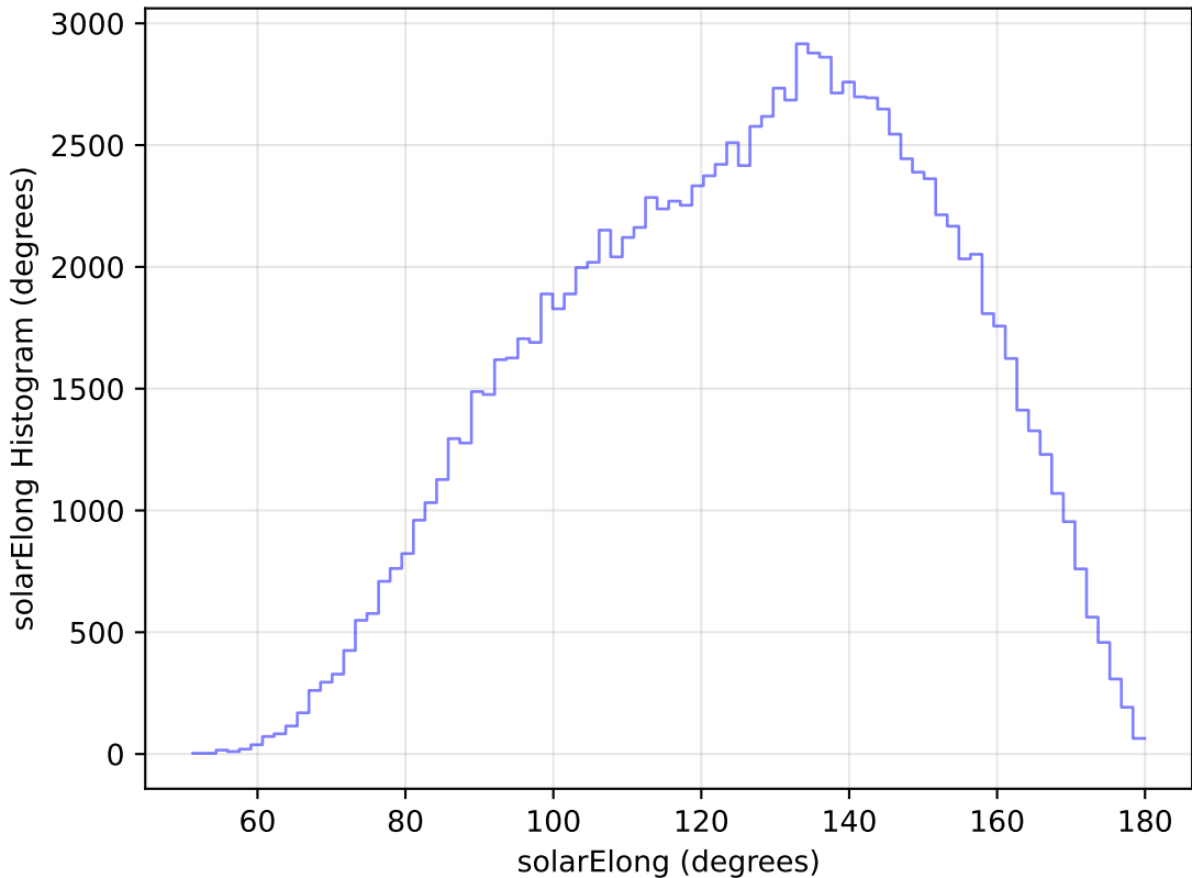
too_ignore_5_1v3.4_10yrs WFD u band: solarElong Histogram
