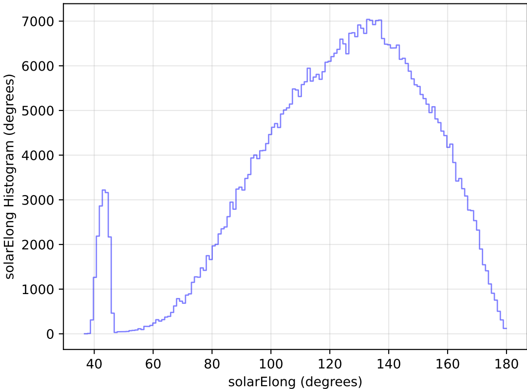
too_ignore_5_1v3.4_10yrs WFD r band: solarElong Histogram
