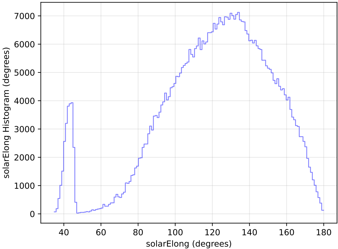
too_ignore_5_1v3.4_10yrs WFD i band: solarElong Histogram
