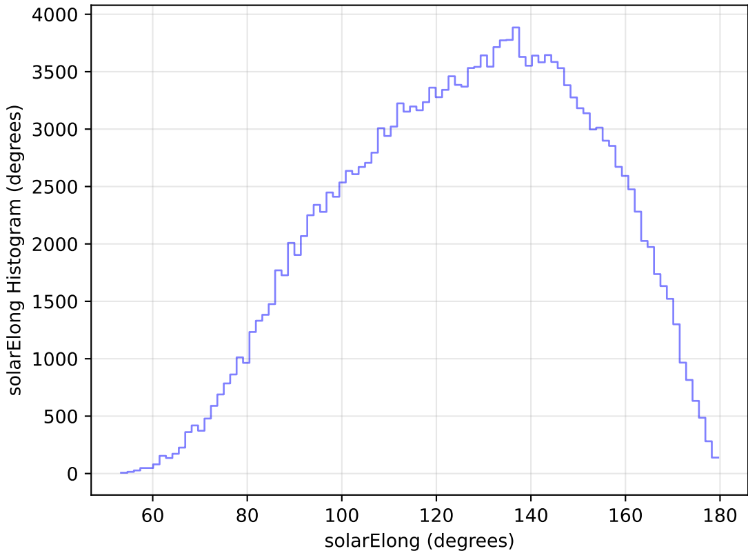
too_ignore_5_1v3.4_10yrs WFD g band: solarElong Histogram
