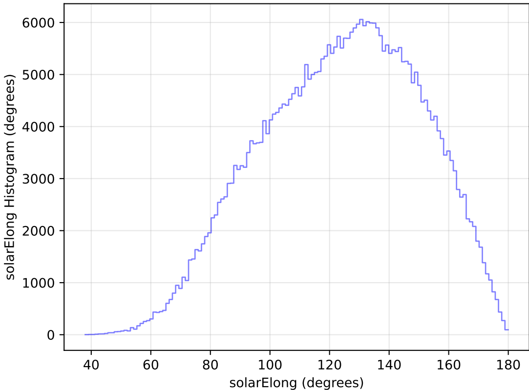
too_ignore_5_1v3.4_10yrs All sky y band: solarElong Histogram
