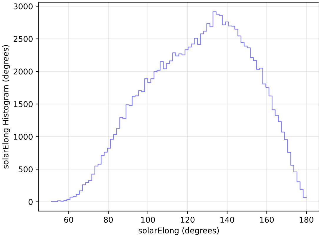
too_ignore_5_1v3.4_10yrs All sky u band: solarElong Histogram
