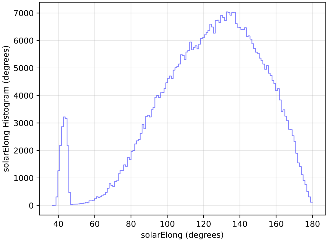
too_ignore_5_1v3.4_10yrs All sky r band: solarElong Histogram
