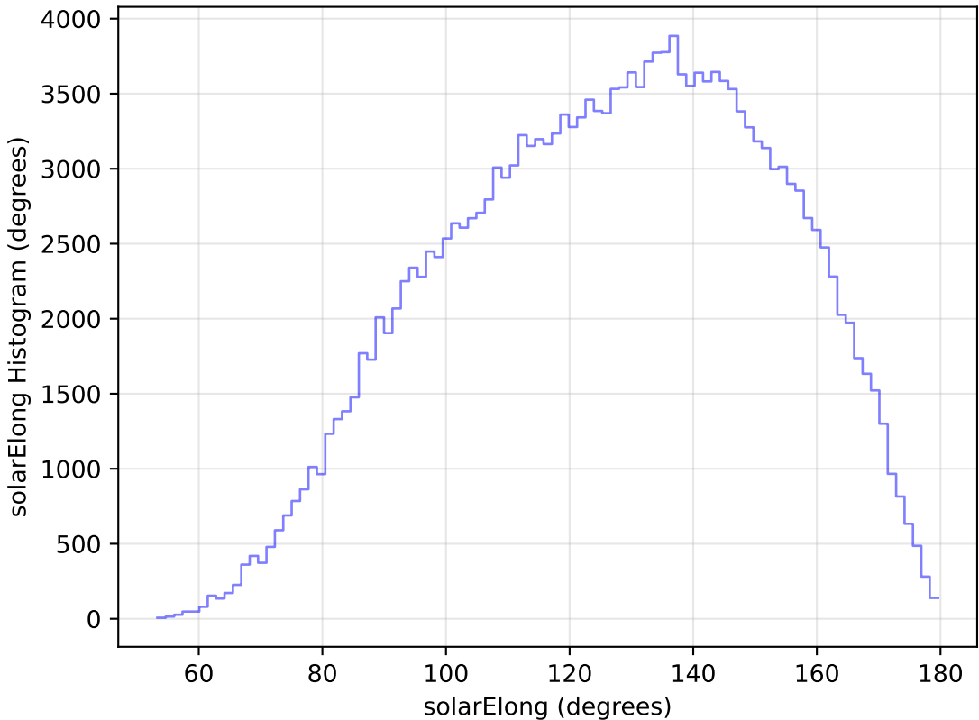
too_ignore_5_1v3.4_10yrs All sky g band: solarElong Histogram
