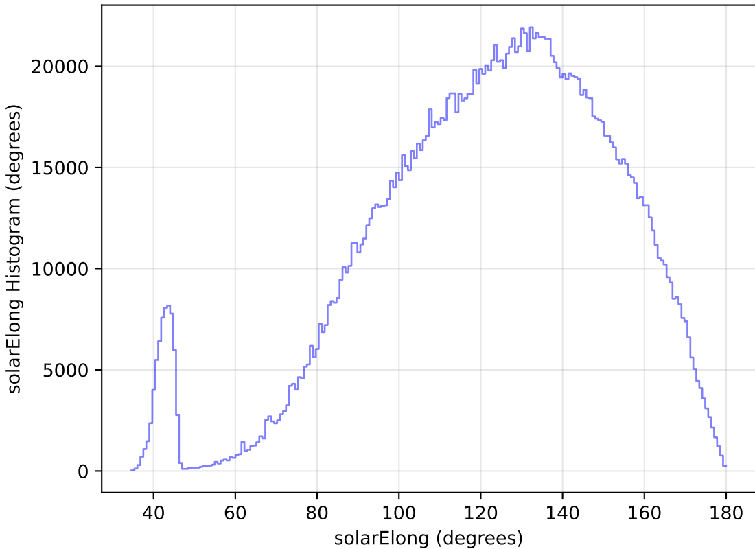
too_ignore_5_1v3.4_10yrs All sky all bands: solarElong Histogram
