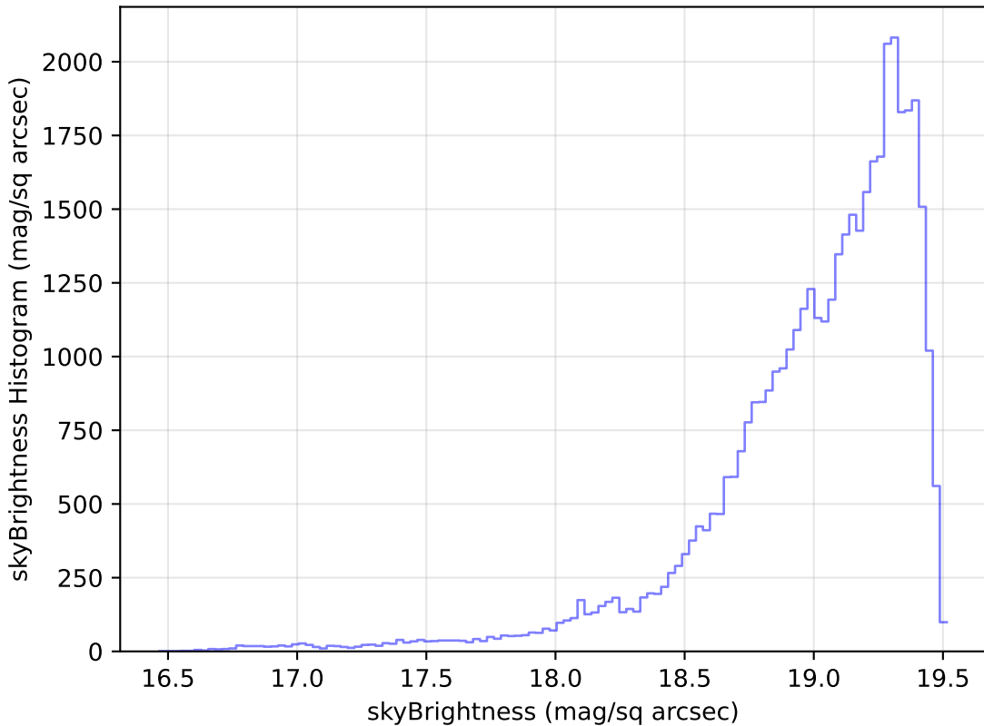
too_ignore_5_1v3.4_10yrs Yr 1 z band: skyBrightness Histogram
