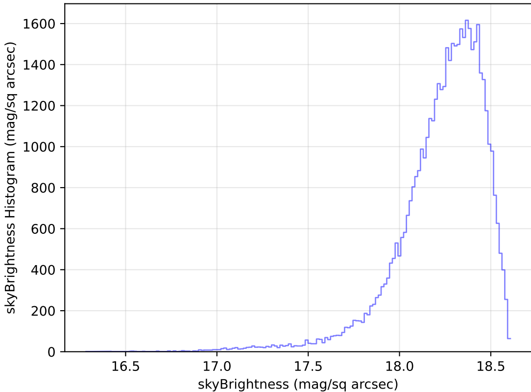
too_ignore_5_1v3.4_10yrs Yr 1 y band: skyBrightness Histogram
