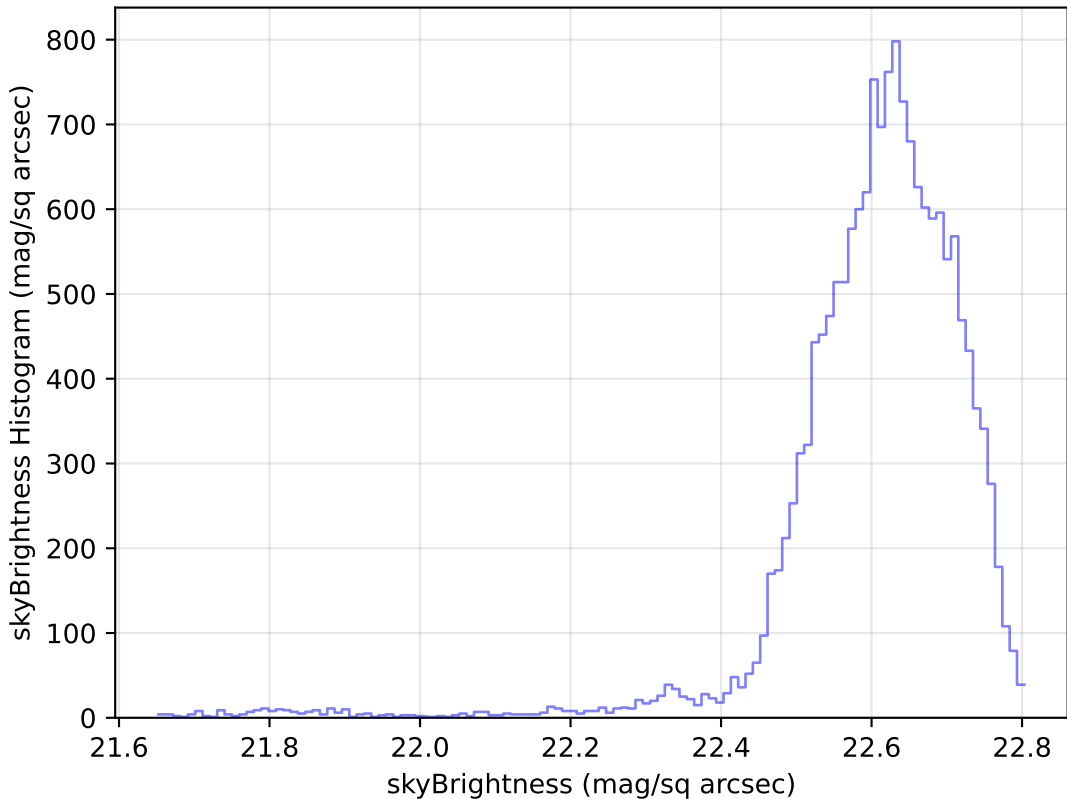
too_ignore_5_1v3.4_10yrs Yr 1 u band: skyBrightness Histogram
