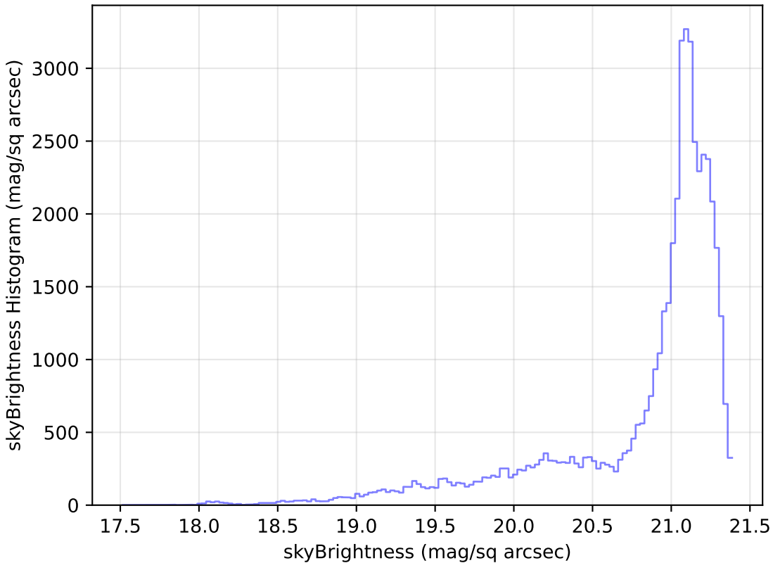
too_ignore_5_1v3.4_10yrs Yr 1 r band: skyBrightness Histogram
