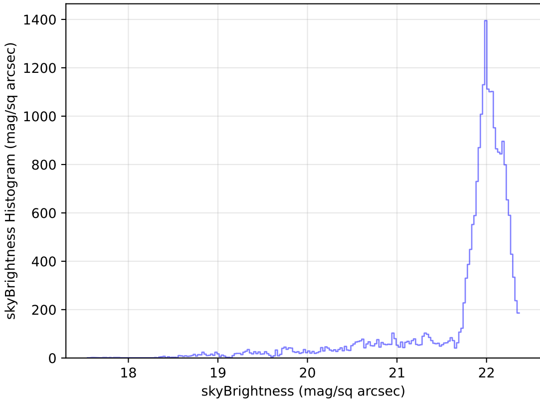
too_ignore_5_1v3.4_10yrs Yr 1 g band: skyBrightness Histogram
