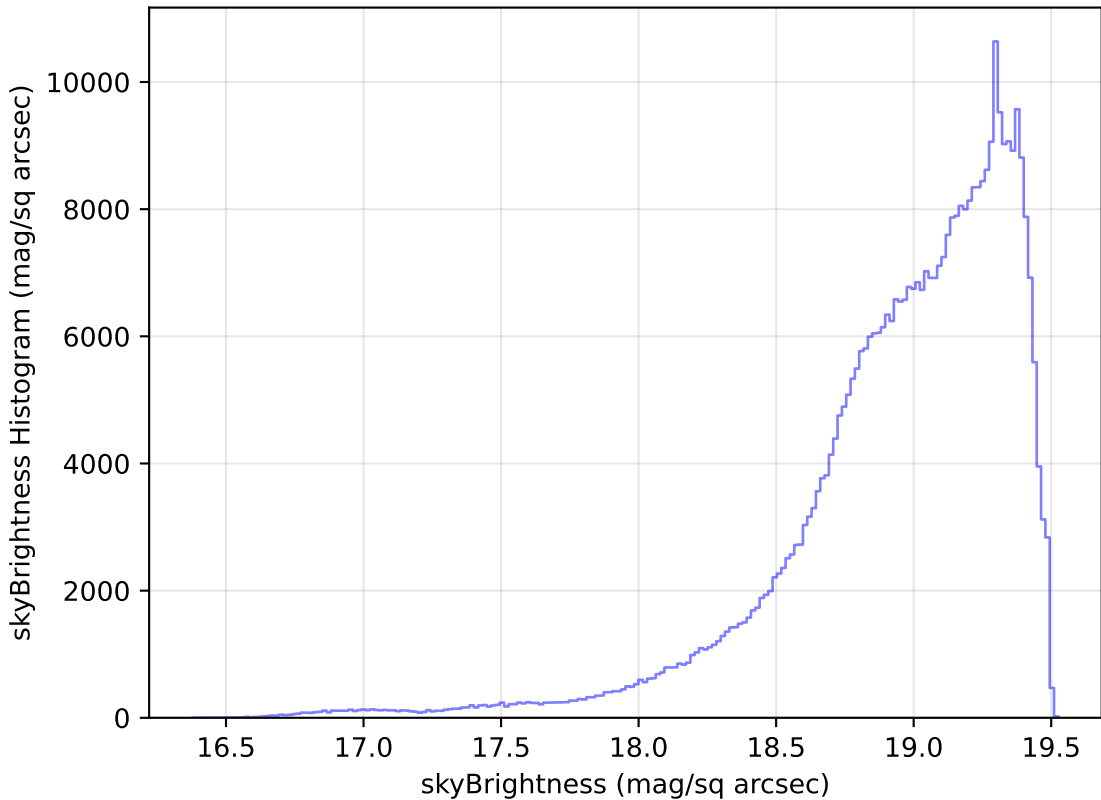
too_ignore_5_1v3.4_10yrs WFD z band: skyBrightness Histogram
