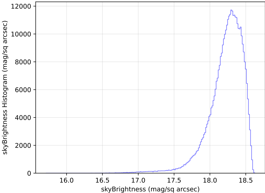
too_ignore_5_1v3.4_10yrs WFD y band: skyBrightness Histogram
