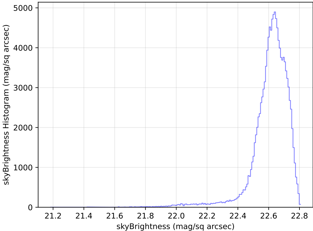
too_ignore_5_1v3.4_10yrs WFD u band: skyBrightness Histogram
