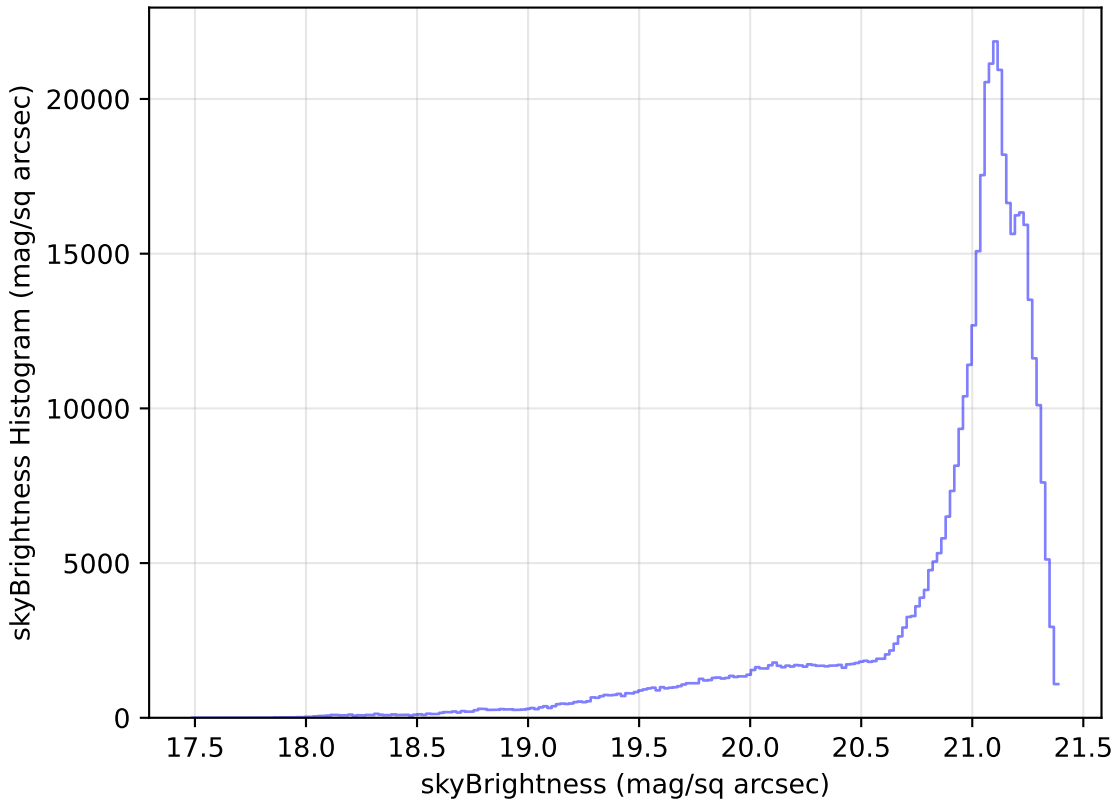
too_ignore_5_1v3.4_10yrs WFD r band: skyBrightness Histogram
