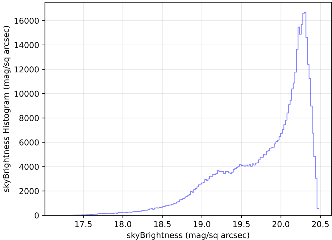
too_ignore_5_1v3.4_10yrs WFD i band: skyBrightness Histogram
