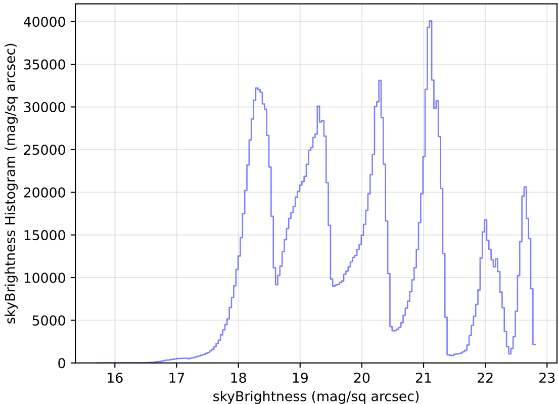
too_ignore_5_1v3.4_10yrs WFD all bands: skyBrightness Histogram
