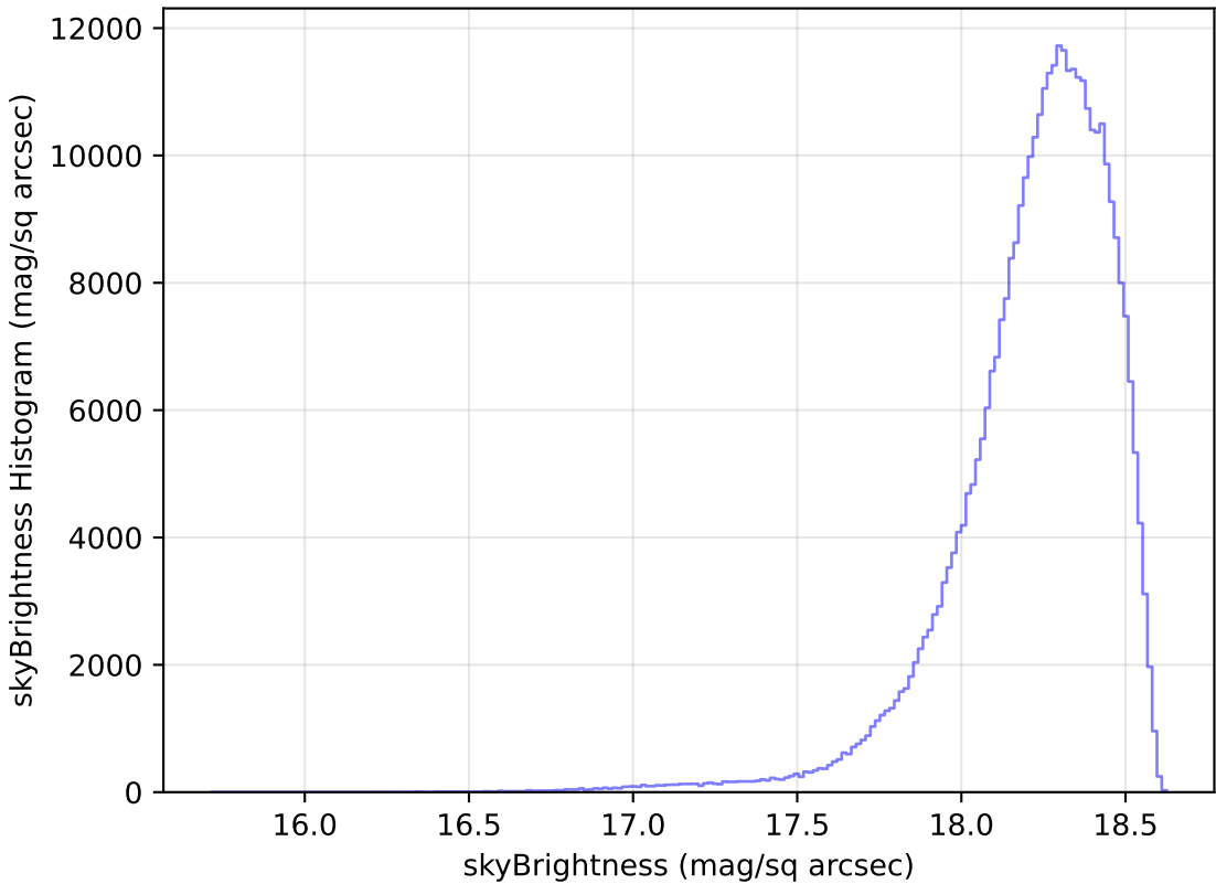
too_ignore_5_1v3.4_10yrs All sky y band: skyBrightness Histogram
