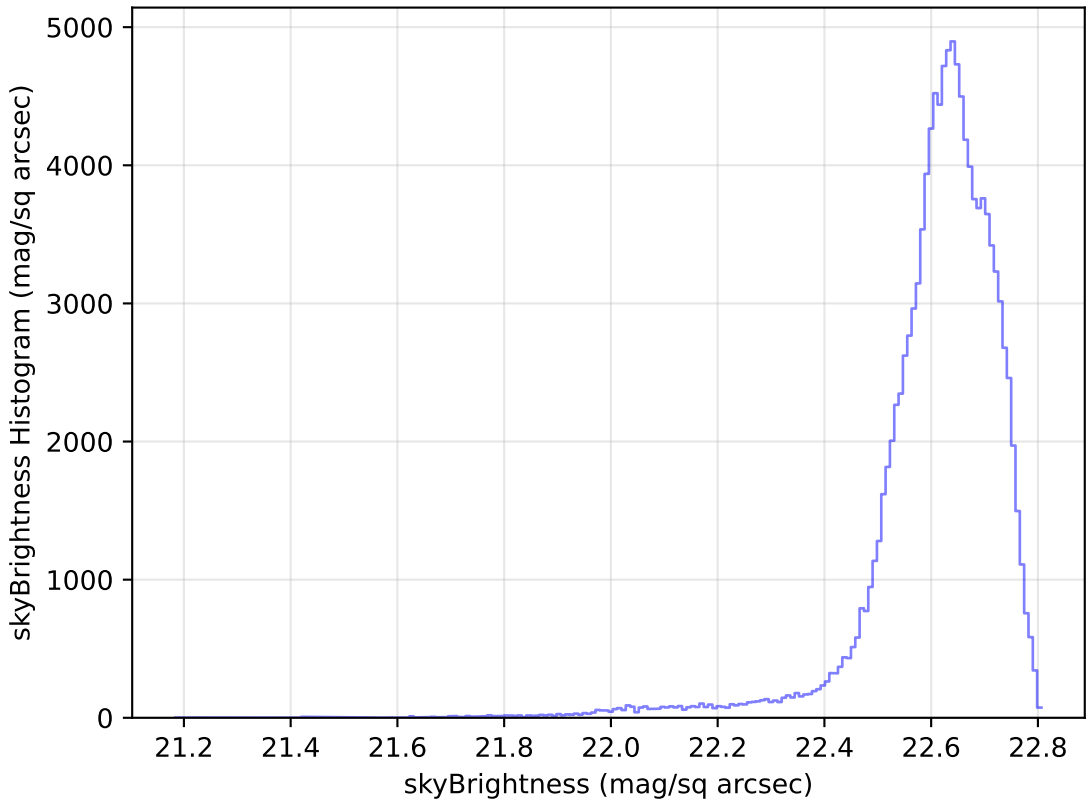
too_ignore_5_1v3.4_10yrs All sky u band: skyBrightness Histogram
