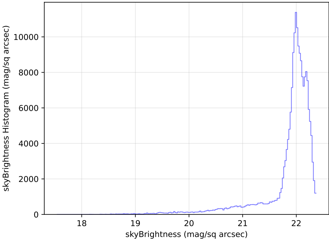
too_ignore_5_1v3.4_10yrs All sky g band: skyBrightness Histogram
