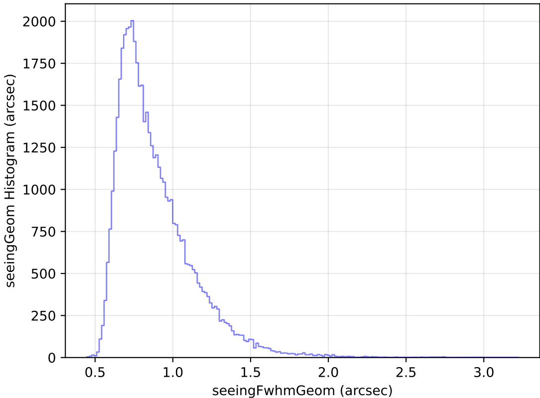
too_ignore_5_1v3.4_10yrs Yr 1 r band: seeingGeom Histogram
